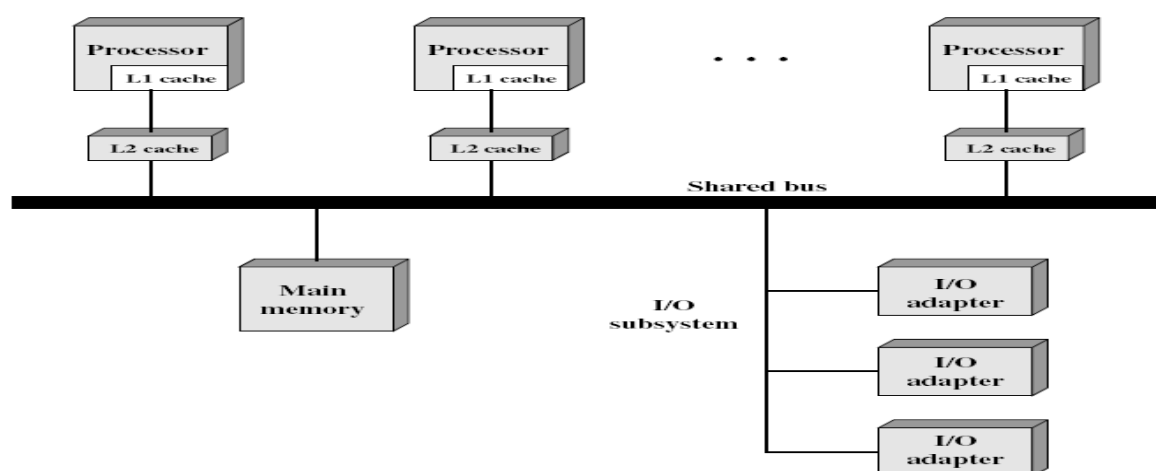
Figure 17.5 Symmetric Multiprocessor Organization
