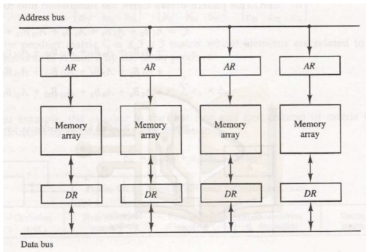
Figure: multiple module memory organization
