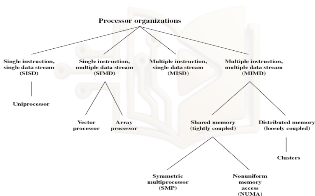
Figure 17.1 A Taxonomy of Parallel Processor Architectures
