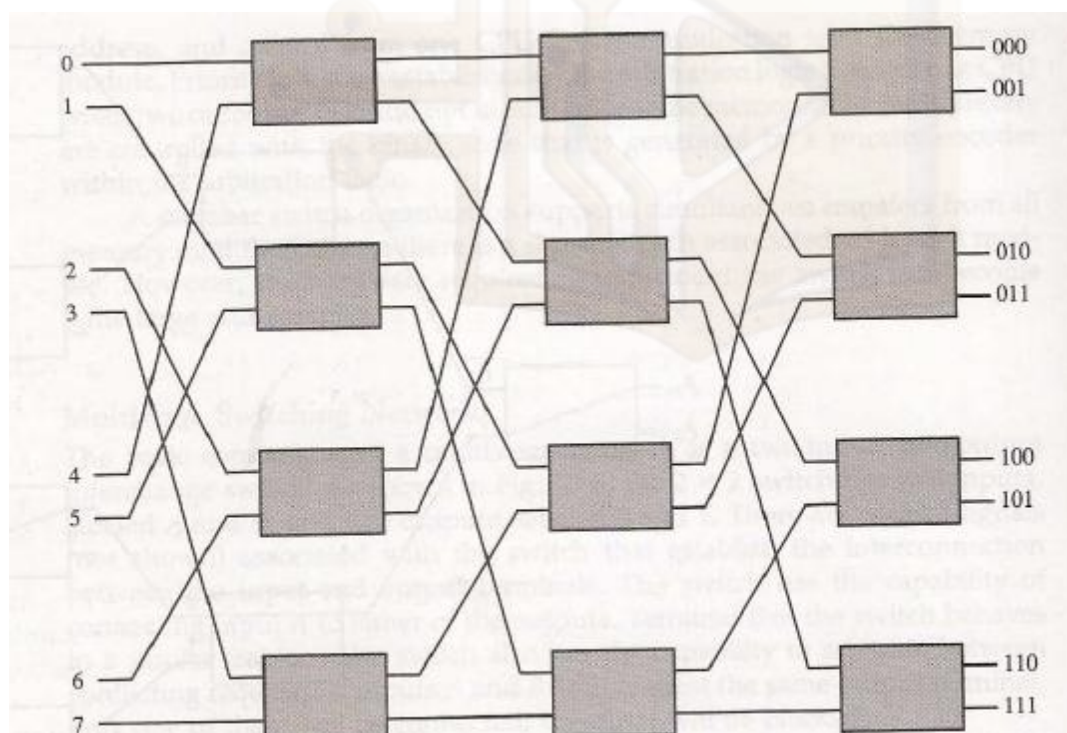
Figure 13-8 8 \times 8 omega switching network.
